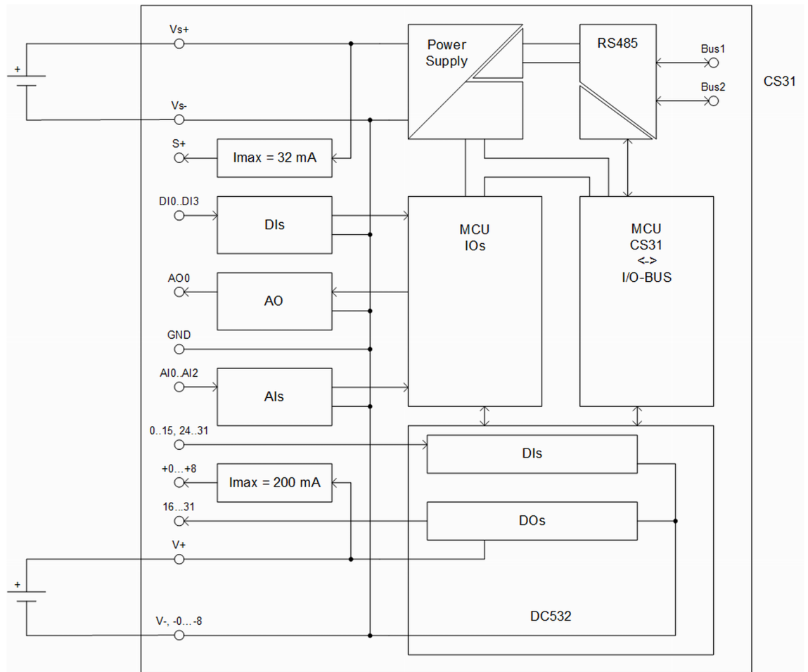
Fig. 76: Schematic diagram
