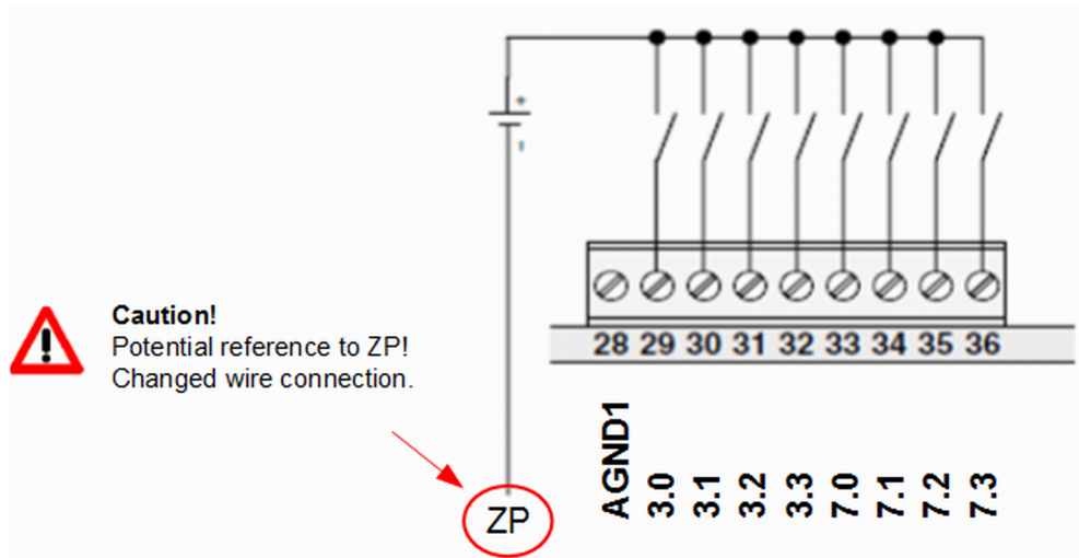
Fig. 23: Use of analog inputs as digital inputs
