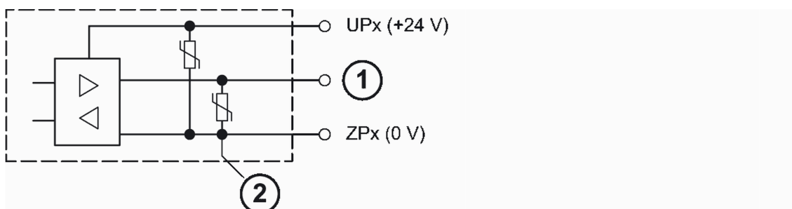
Fig. 16: Circuitry of a digital input/output with varistors for demagnetization when switching off inductive loads
