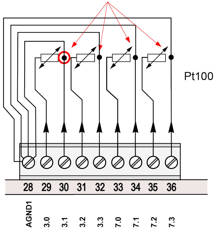
Fig. 22: Connection of Pt100 temperature sensors in 3-wire configuration
