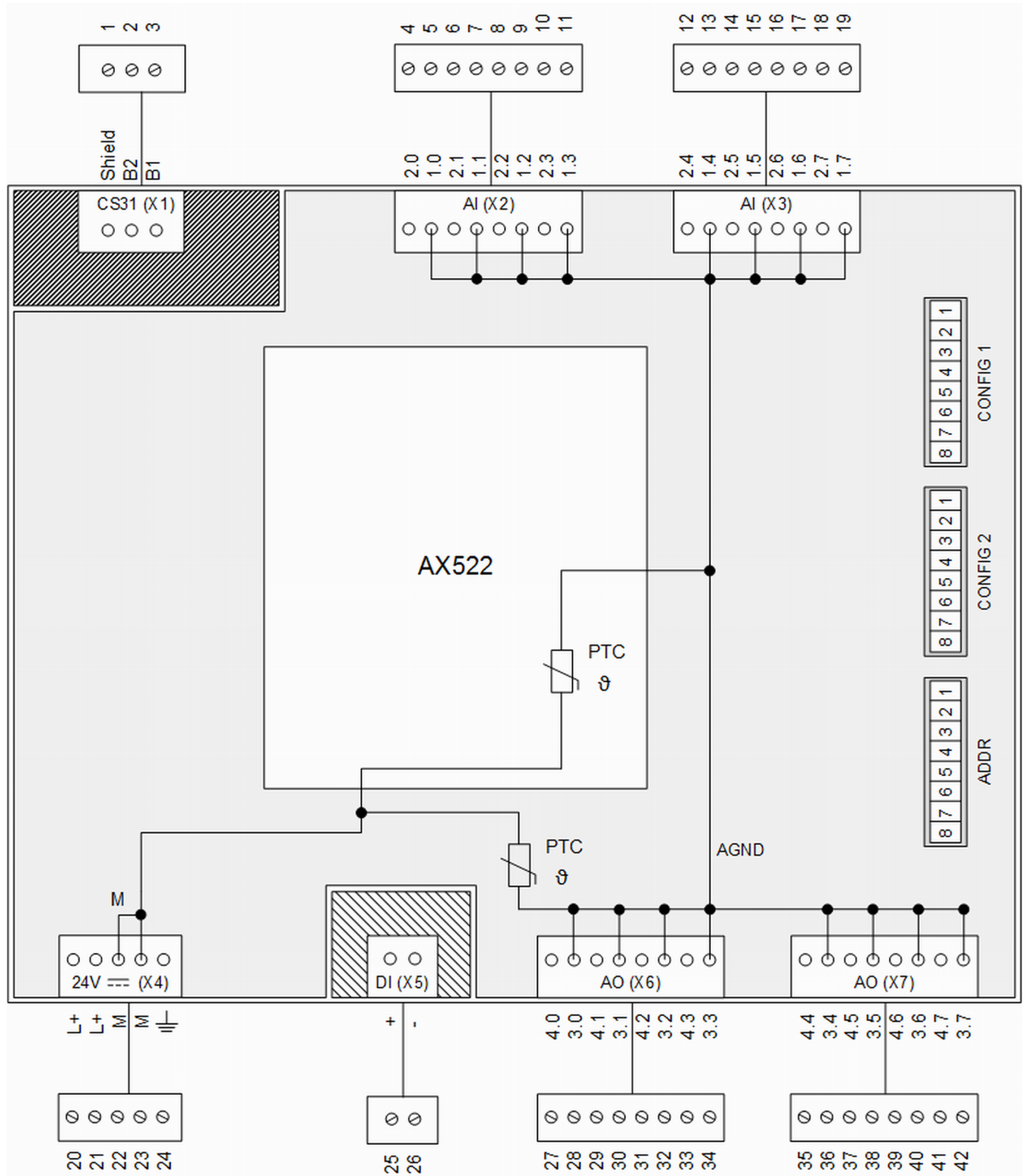
Fig. 34: Connection
