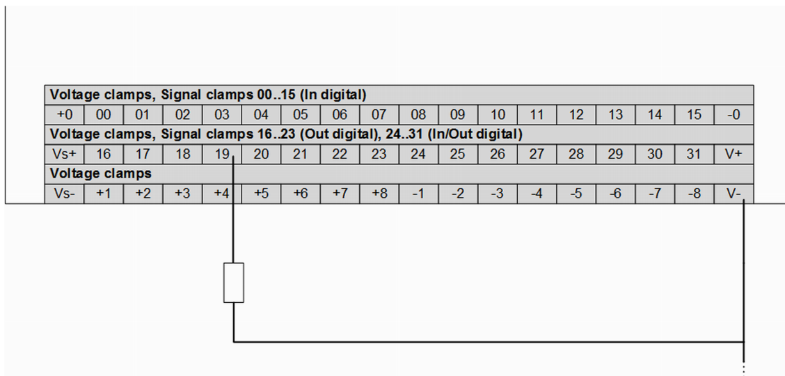
Fig. 71: Connection example: digital output
