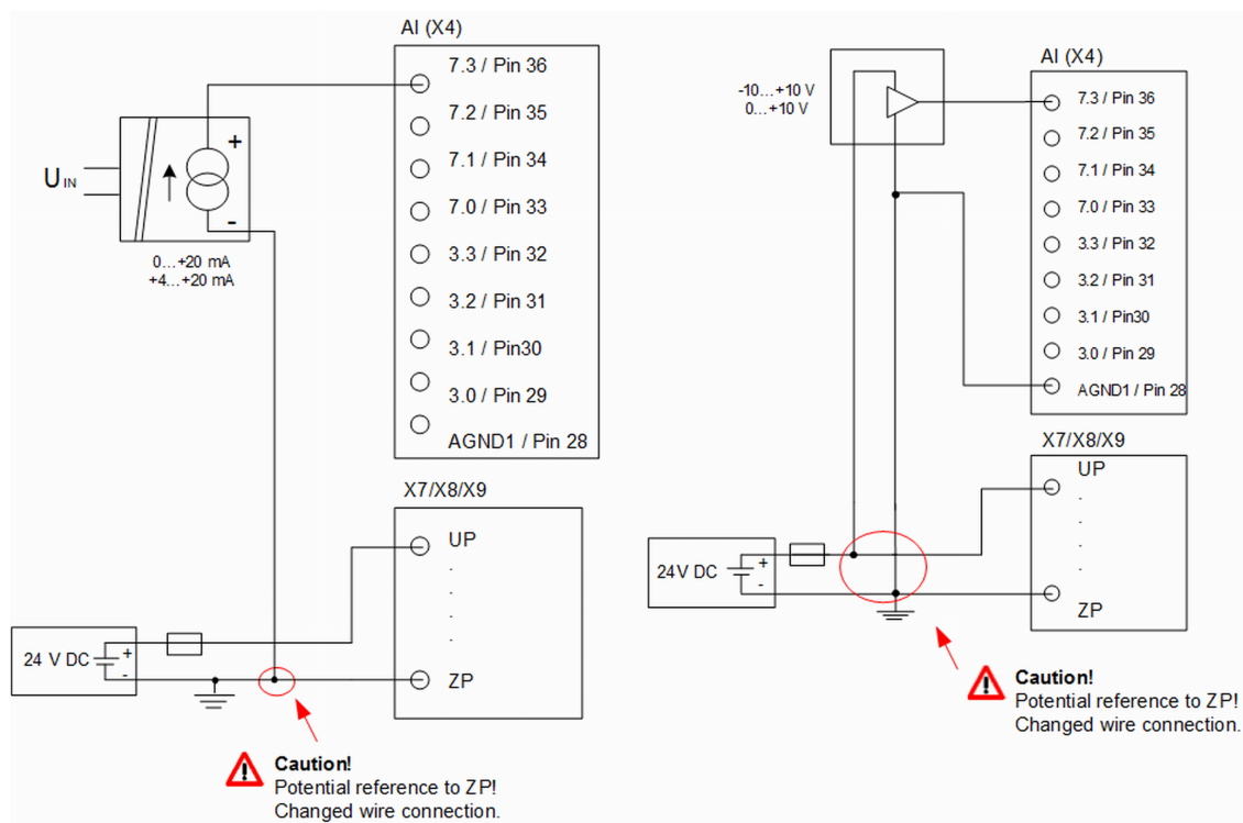
Fig. 21: Connection of current sensors 0 mA ... 20 mA to the analog inputs
