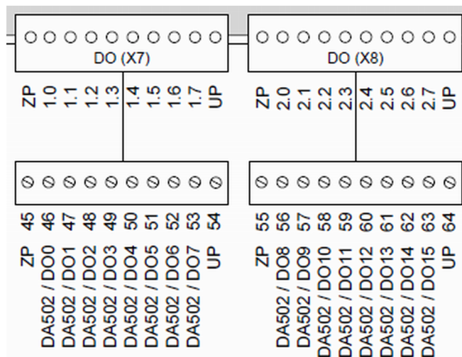
Fig. 14: Arrangement of digital outputs
