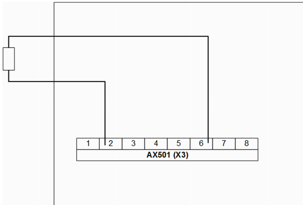
Fig. 74: Connection example: Voltage output
