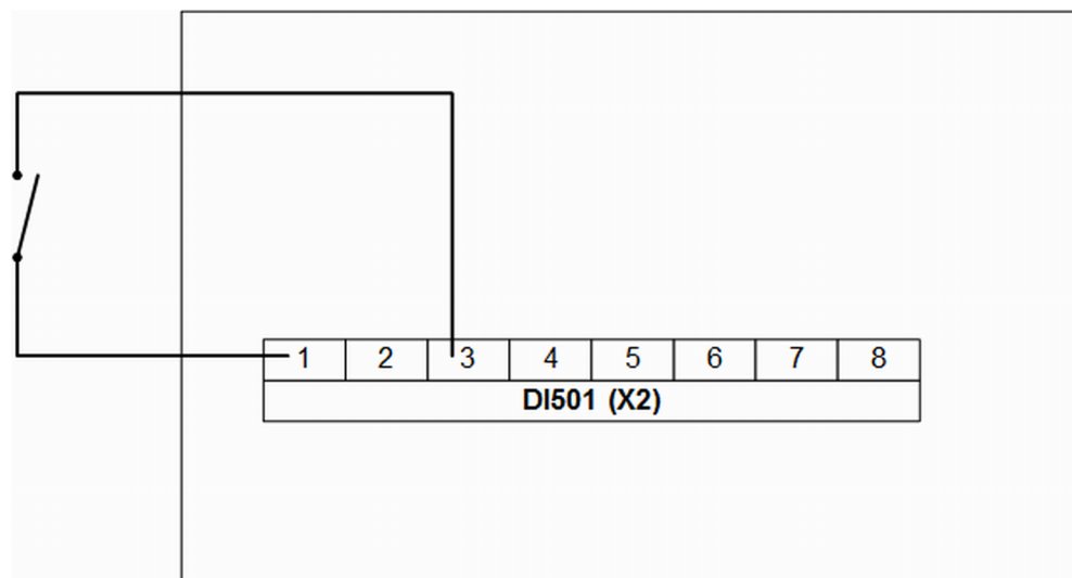
Fig. 72: Connection example: digital input (X2)
