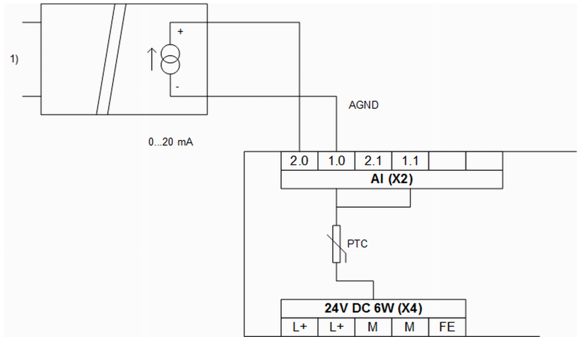
Fig. 36: Current input
