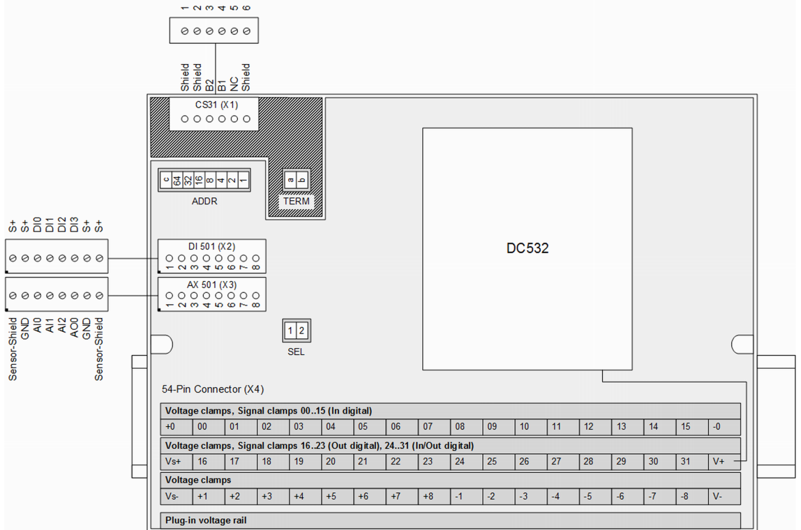
Fig. 69: Connection
