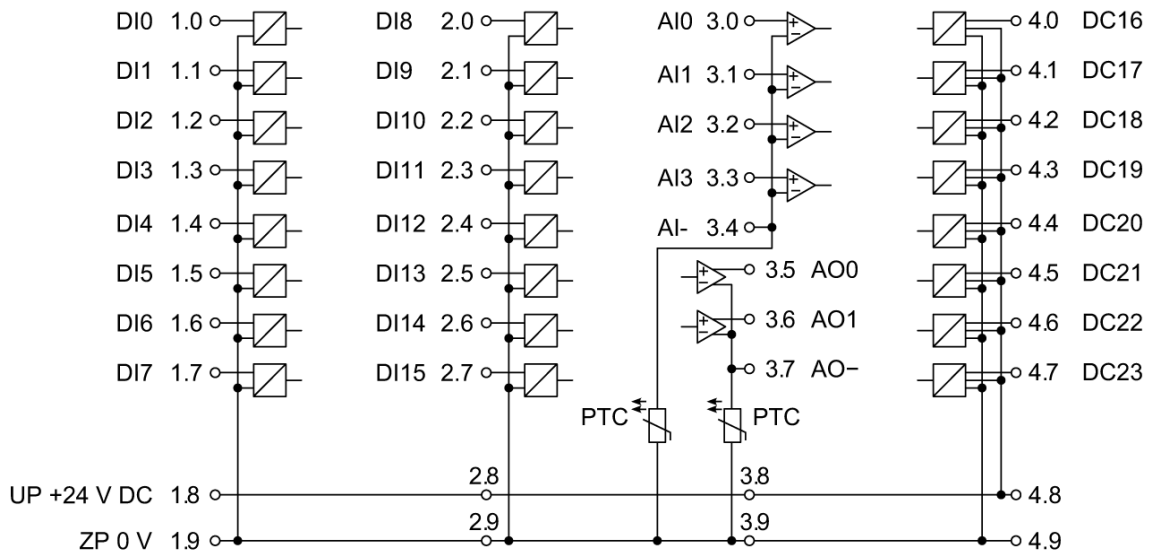
Fig. 13: Circuit arrangement of DA501 module
