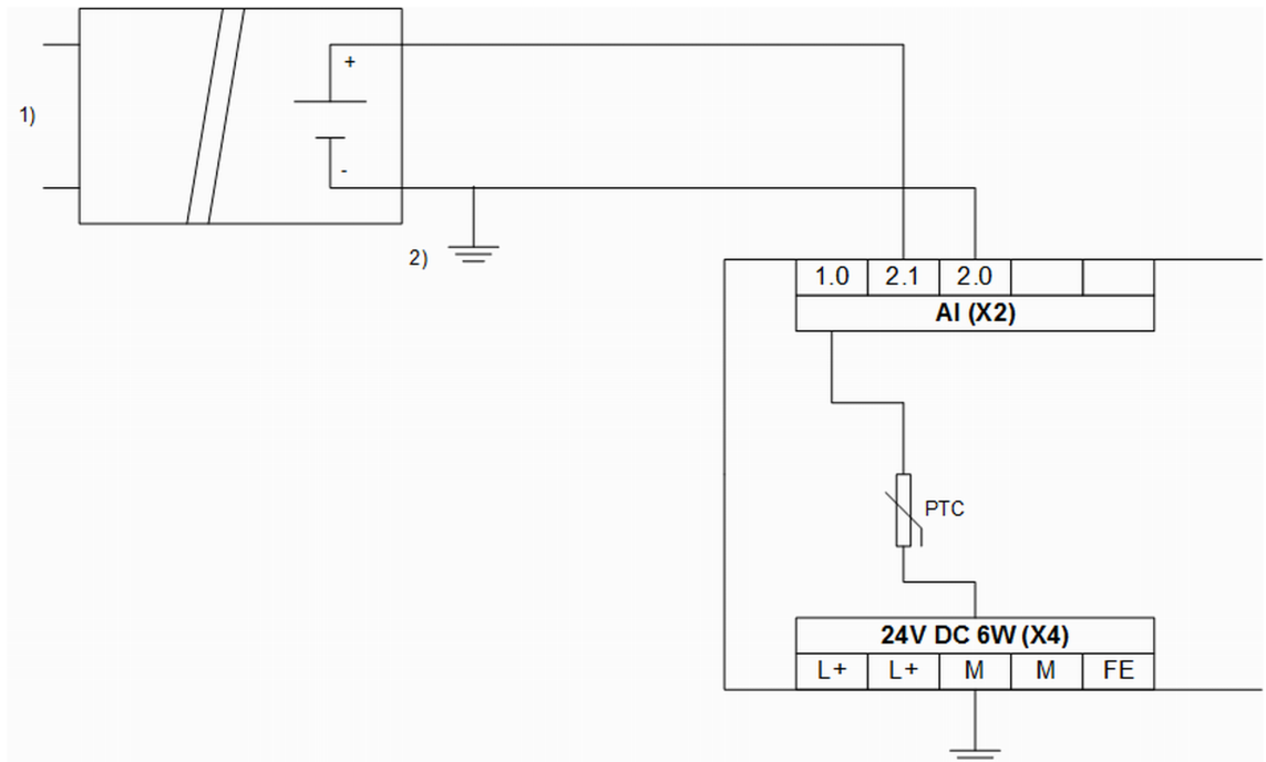
Fig. 43: Differential voltage input
