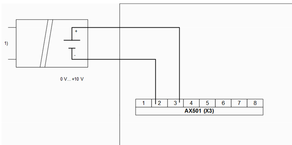
Fig. 73: Connection example: Voltage input
