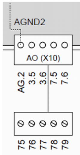
Fig. 24: Arrangement of the analog outputs
