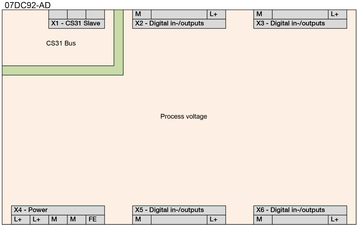
Fig. 65: Process voltage connections - 07DC92-AD
