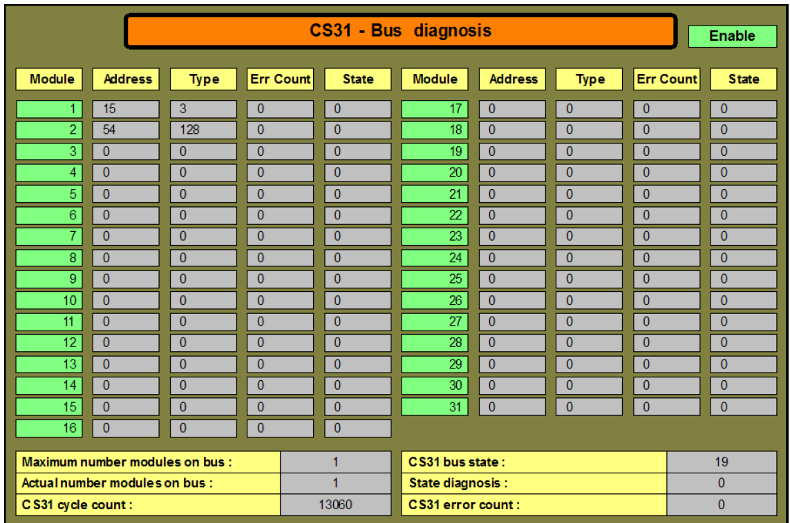
Fig. 7: Visualization: CS31 bus diagnosis
